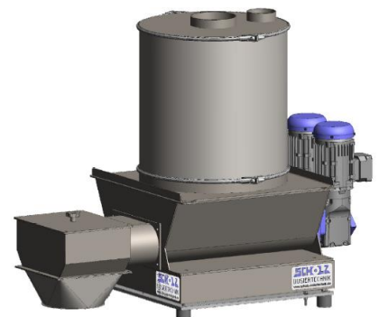
GOLO with 100-liter-hopper and vertical tube-outlet, placed on platform-scale BASIC600
