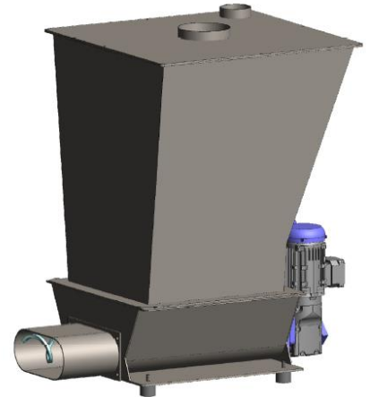
GOLO with 280-liter-hopper and horizontal tube-outlet
