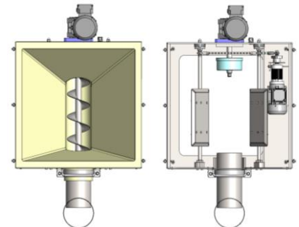
Top view with / without PU-hopper
